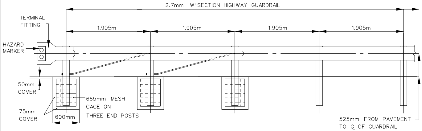
ELEVATION BREAKAWAY CABLE TERMINAL
