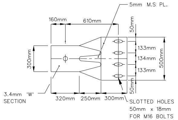
BRIDGE END POST
