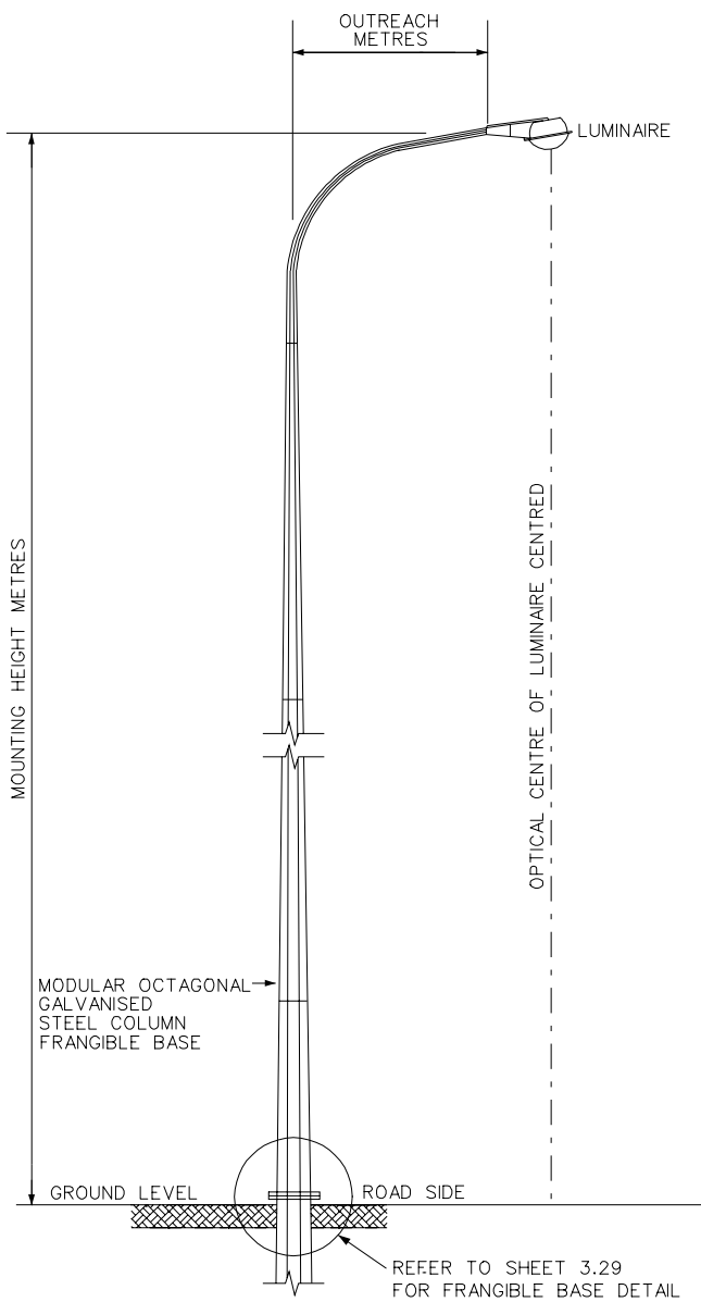
STREETLIGHTING COLUMN FRANGIBLE BASE (speed limits greater than 50 km/h)
