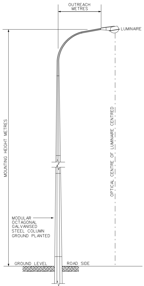
STREETLIGHTING COLUMN GROUND PLANTED (speed limits 50 km/h or less)
